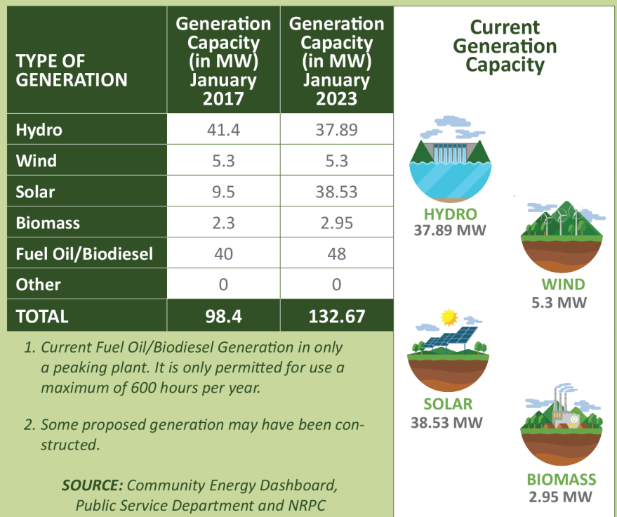
FIGURE 4: Regional Generation Capacity
