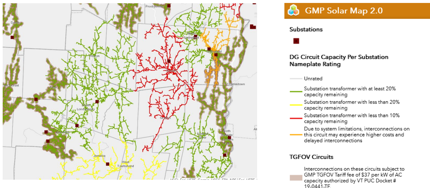
FIGURE 19: GREEN MOUNTAIN SOLAR HOSTING CAPACITY MAPS
